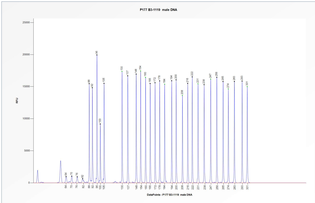
Figure 1. Capillary electrophoresis pattern from a sample of approximately 50 ng human male control DNA analysed with SALSA MLPA Probemix P177 CASR (B3-1119).
