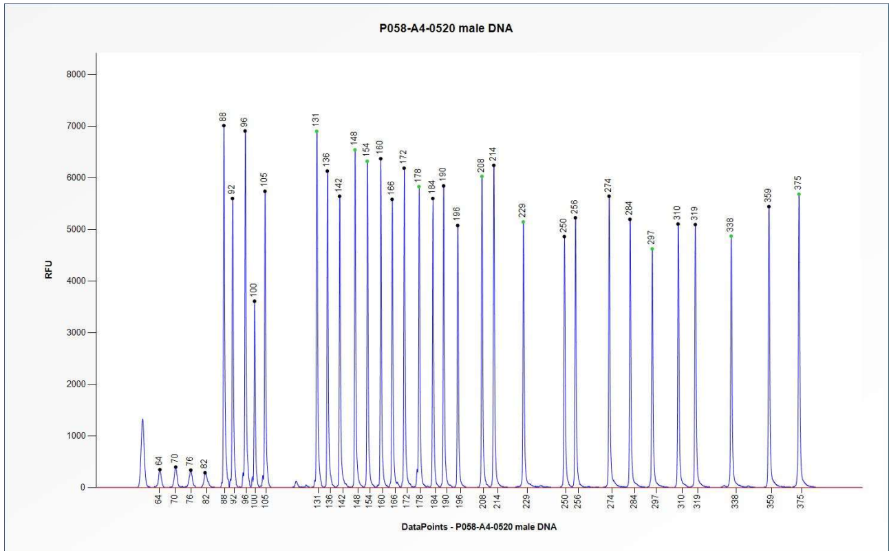
Figure 1. Capillary electrophoresis pattern from a sample of approximately 50 ng human male control DNA analysed with SALSA MLPA Probemix P058 IGHMBP2 (A4-0520).
