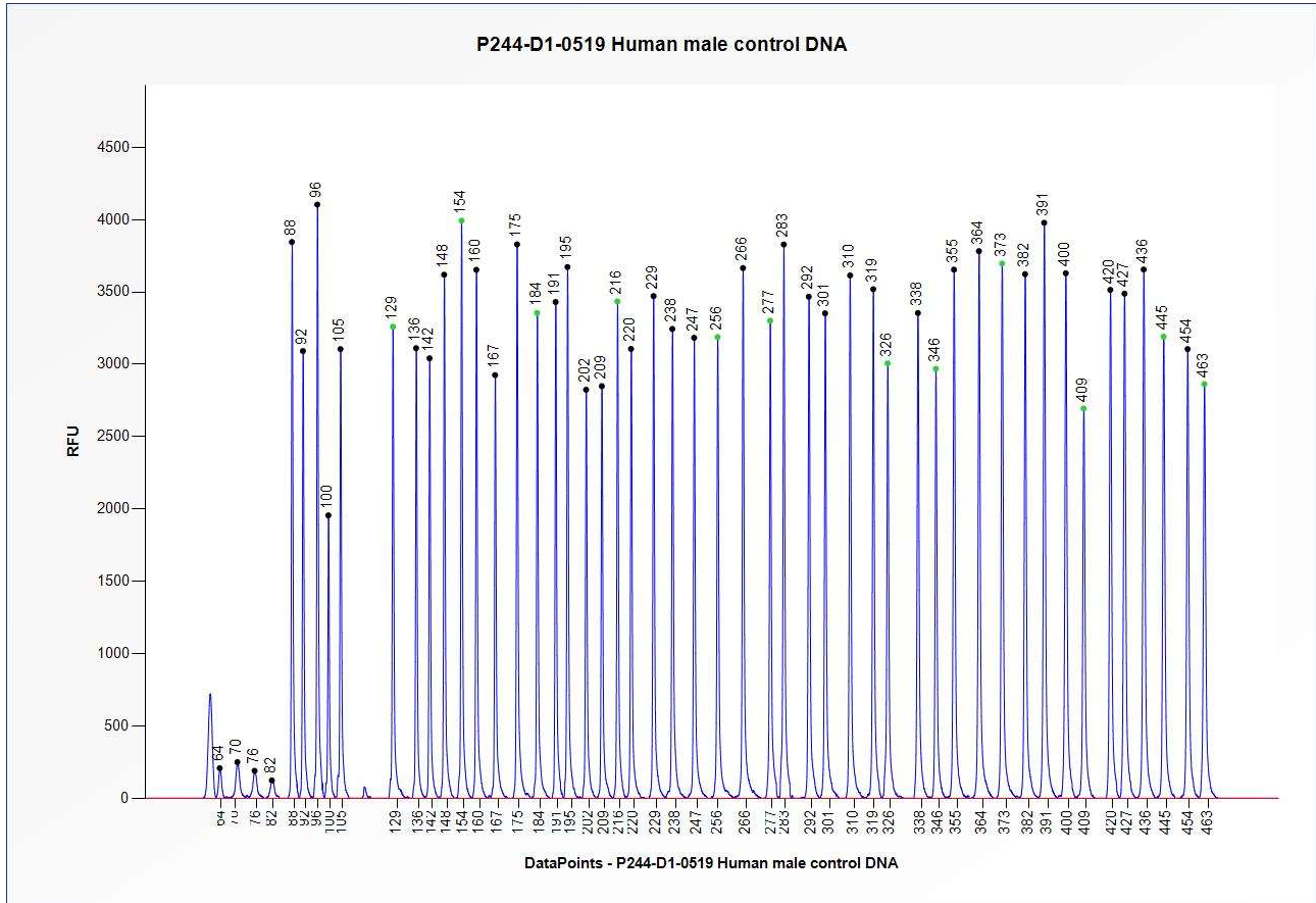
Figure 1. Capillary electrophoresis pattern from a sample of approximately 50 ng human male control DNA analysed with SALSA MLPA Probemix P244 AIP-MEN1-CDKN1B (D1-0519).
