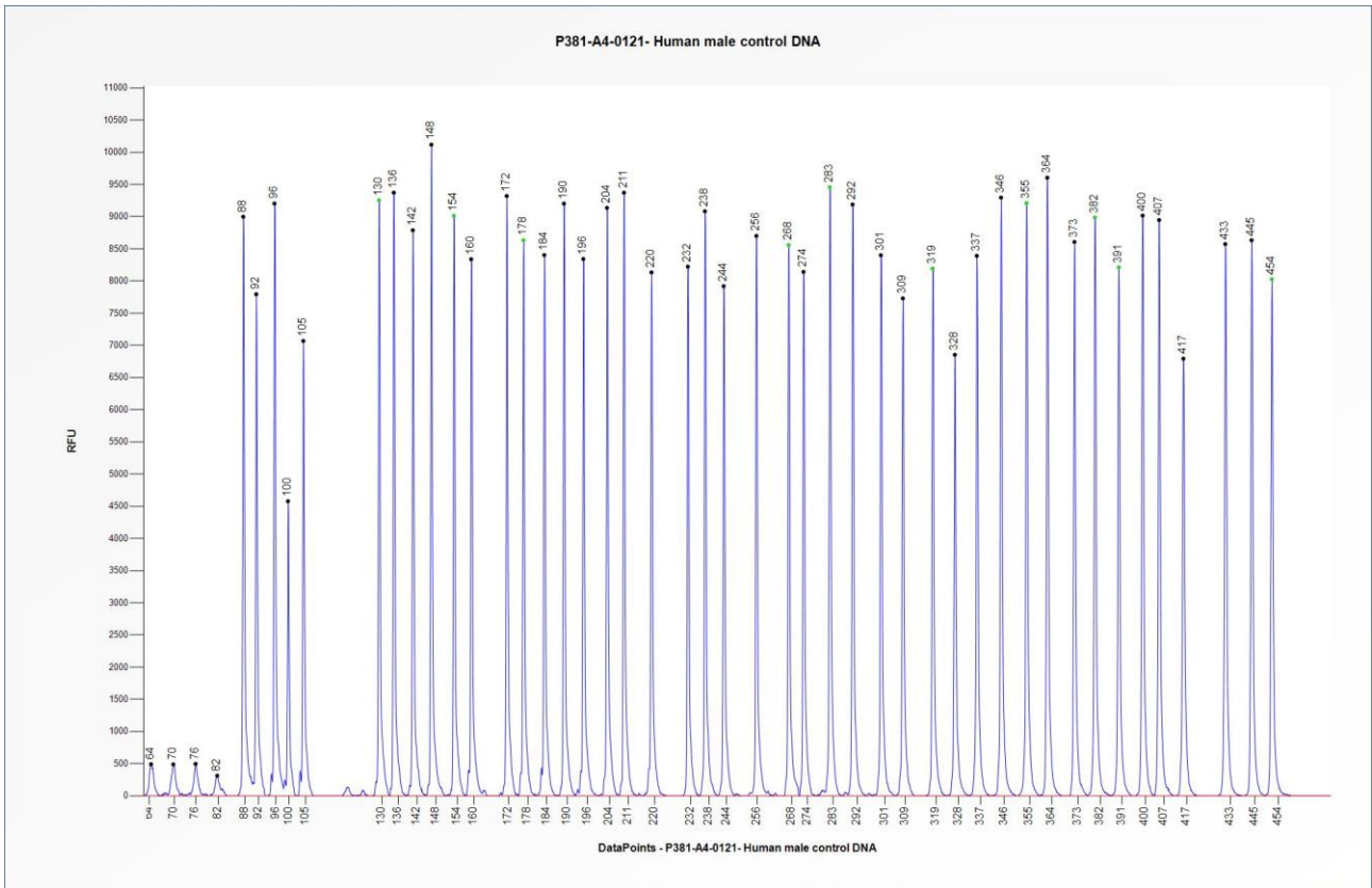
Figure 1. Capillary electrophoresis pattern from a sample of approximately 50 ng human male control DNA analysed with SALSA MLPA Probemix P381 COL11A1 mix 1 (A4-0121).
