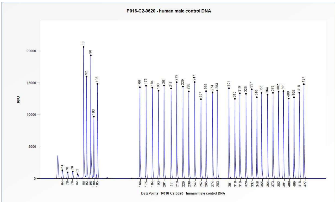
Figure 1. Capillary electrophoresis pattern from a sample of approximately 50 ng human male control DNA analysed with SALSA MLPA Probemix P016 VHL (C2-0620).
