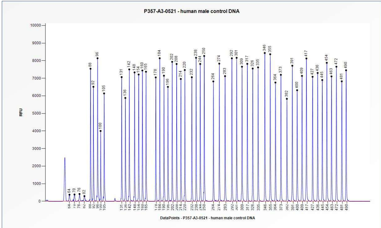
Figure 1. Capillary electrophoresis pattern from a sample of approximately 50 ng human male control DNA analysed with SALSA MLPA Probemix P357 MODY Mix 2 (A3-0521).
