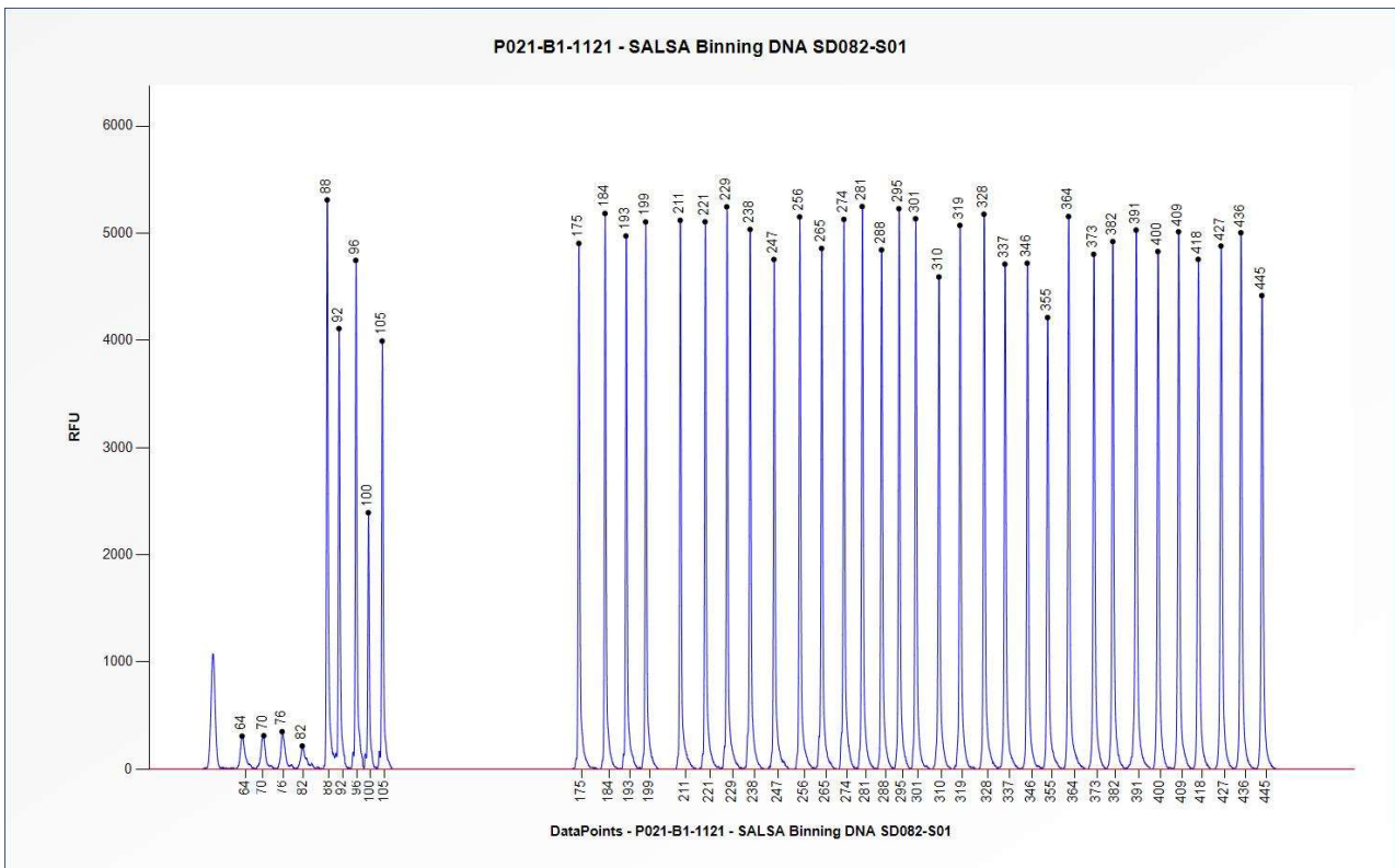
Figure 2. Capillary electrophoresis pattern from SALSA Binning DNA SD082-S01 (approximately 50 ng) analysed with SALSA MLPA Probemix P021 SMA (B1-1121).
