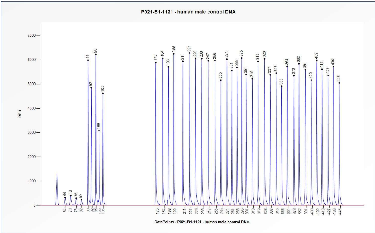
Figure 1. Capillary electrophoresis pattern from a sample of approximately 50 ng human male control DNA analysed with SALSA MLPA Probemix P021 SMA (B1-1121).
