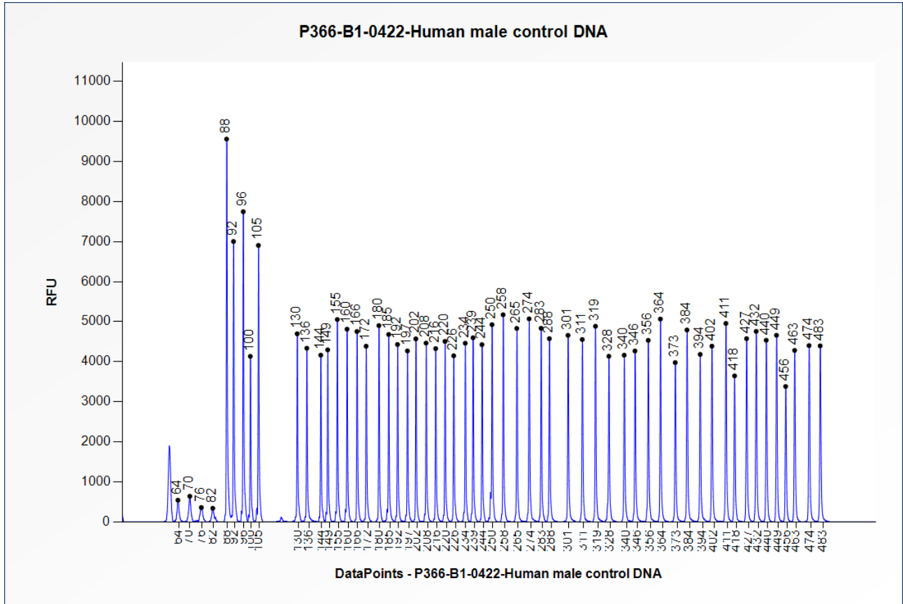
Figure 1. Capillary electrophoresis pattern from a sample of approximately 50 ng human male control DNA analysed with SALSA MLPA Probemix P366 CHM-RP2-RPGR (B1-0422).
