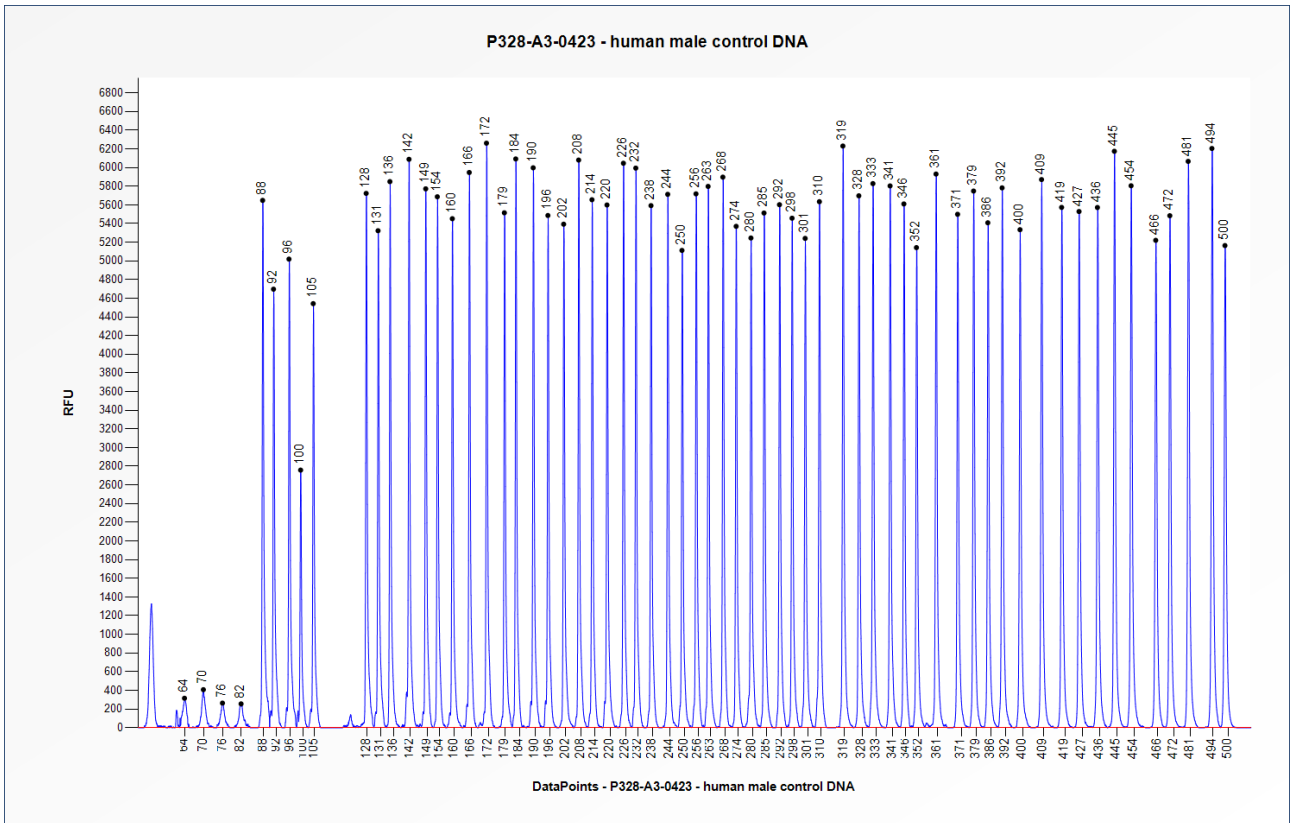
Figure 1. Capillary electrophoresis pattern from a sample of approximately 50 ng human male control DNA analysed with SALSA MLPA Probemix P328 EYS (A3-0423).
